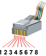
8-pin RJ45 Connector (8P8C)
