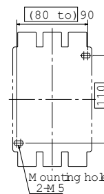
Panel drilling
