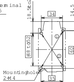
Panel drilling
